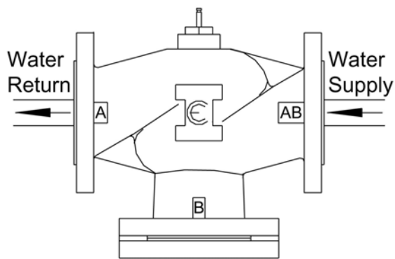
Fig. 1 Two-way valve
